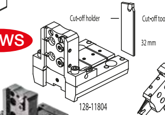
Face and O.D. cutting holder Polygonal
