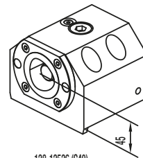
Boring bar holder Polygonal
