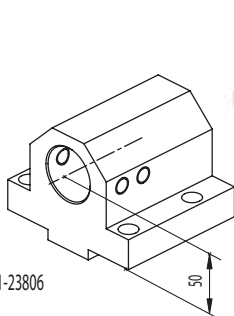
Toolholder for insertdrill with internal coolant Ø40 mm
