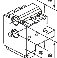
Boring bar holder Ø32 mm
