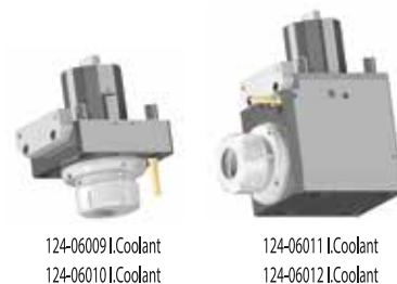
Face and O.D. cutting holder Polygonal
